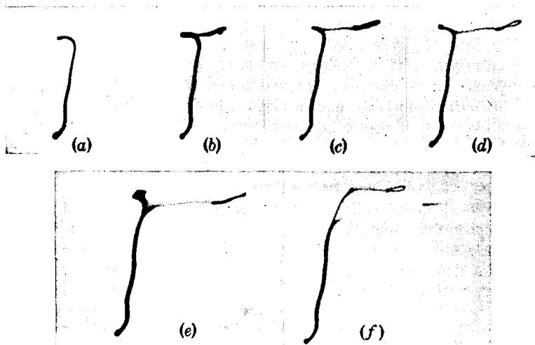
FIG. 8-17.— (V,I) -traces of a mode skip arranged in order of increasing voltage. Only the trace corresponding to the rising edge of the pulse is shown. (a) Below oscillations; (b) beginning of oscillations; (c) middle of oscillation region; (d) beginning of misfiring; (e) misfiring into the nonoscillating state; (f) misfiring into a higher-voltage mode.
